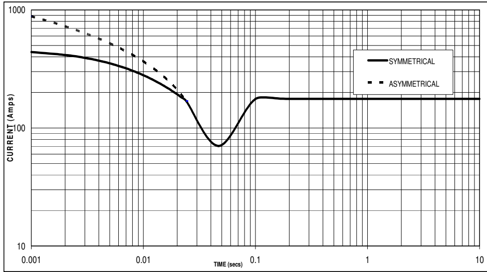
Sustained Short Circuit = 176 Amps
