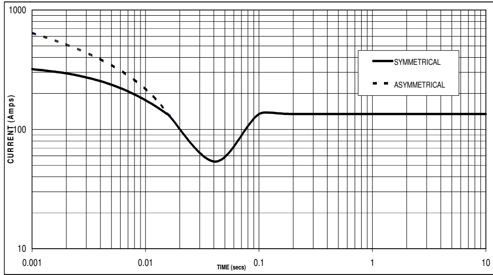
Sustained Short Circuit = 134 Amps
