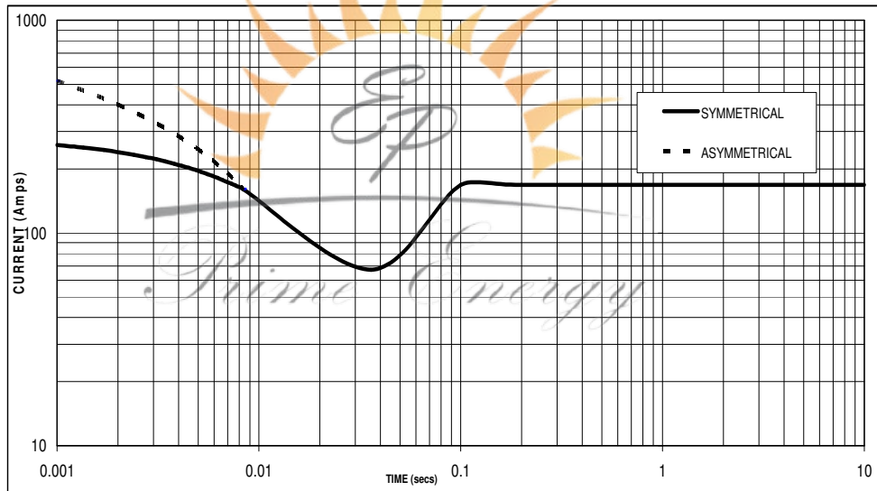
Sustained Short Circuit = 168 Amps
