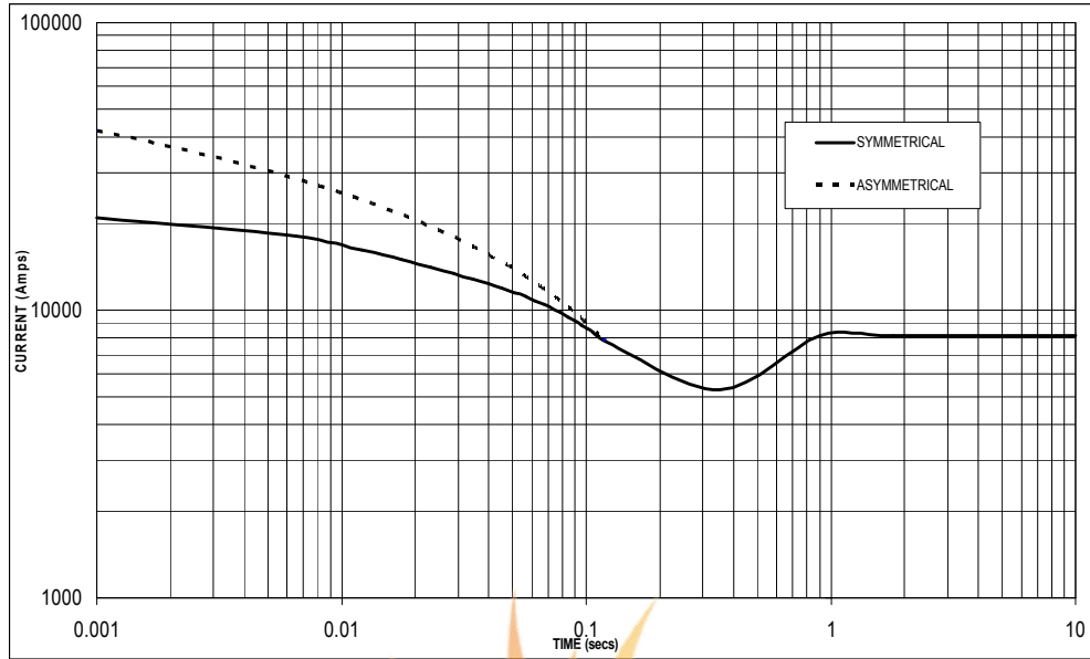
Sustained Short Circuit = 8,150 Amps
